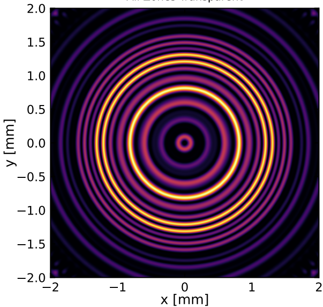
All Zones Transparent
